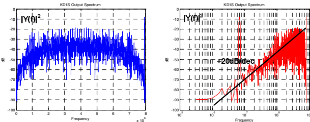
Figure 6 Simulation results (PSD of the output with linear and log frequency axes) for KD1S modulator with ideal components.
