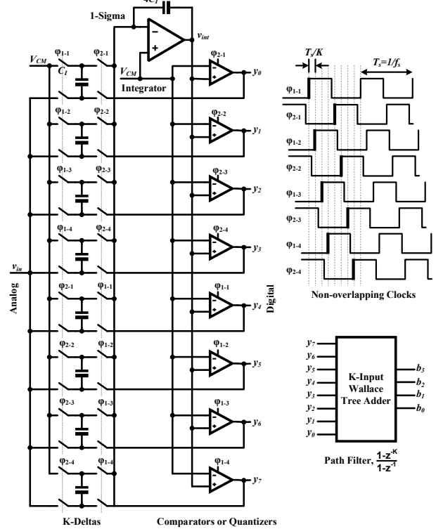
Figure 3 The K -Delta-1-Sigma modulator topology.
