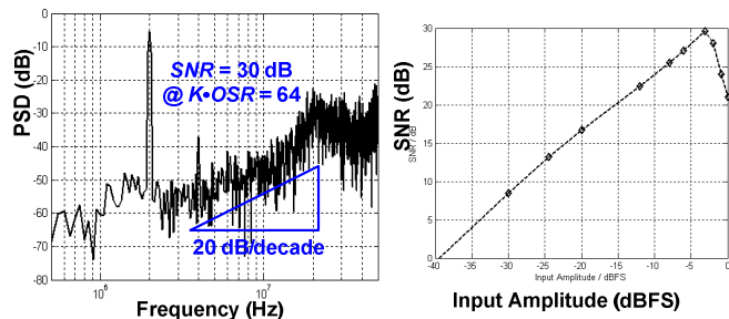
Figure 10 Measured Spectrum and SNR vs. input amplitude plot for the KD1S modulator.
